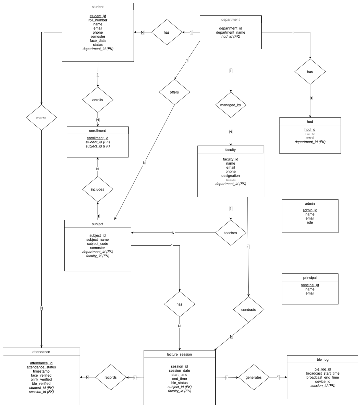
ER Diagram – Face Recognition based Attendance System
