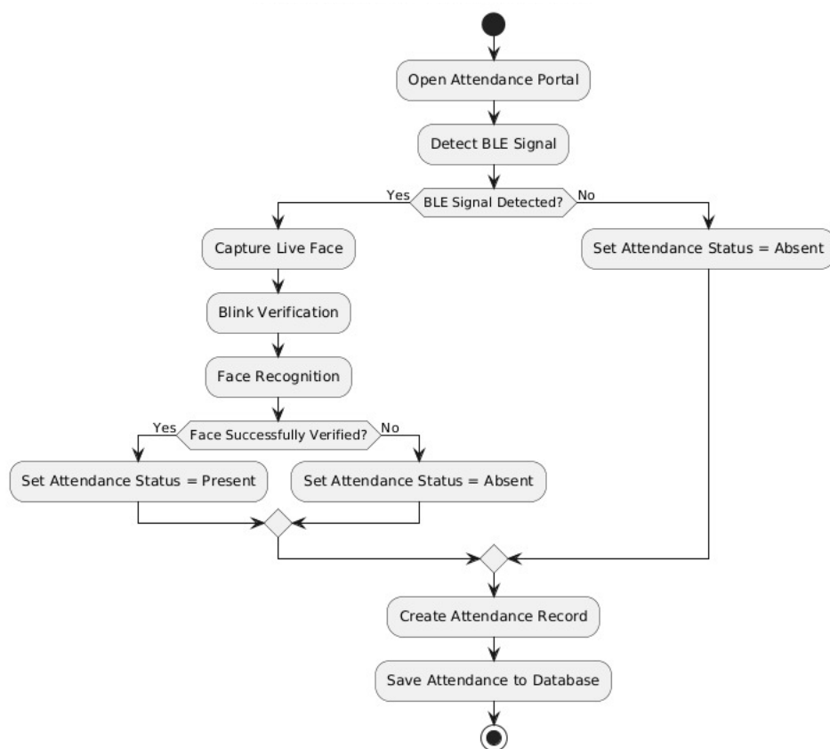
Activity Diagram – Face Recognition based Attendance System
