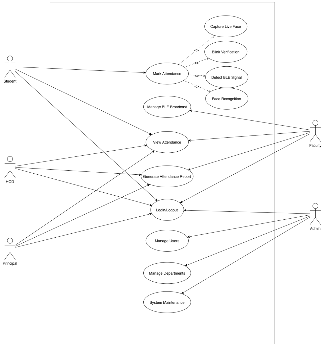
Use case Diagram – Face Recognition based Attendance System
