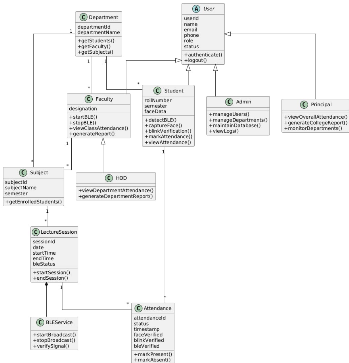
Class Diagram – Face Recognition based Attendance System
