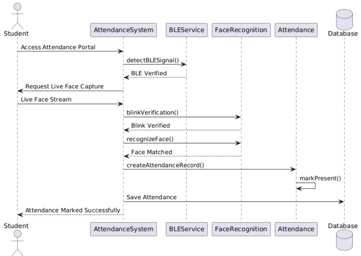
Sequence Diagram – Face Recognition based Attendance System
